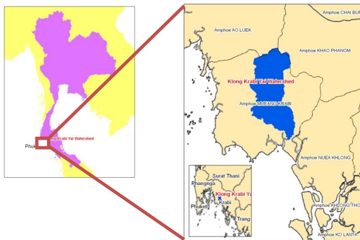
Figure1. Klong Krabi Yai watershed (blue)
